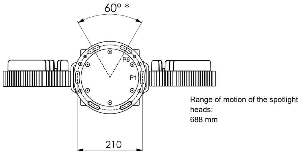
Figure 4 Mounting holes (hole circle Ø 210 mm)
