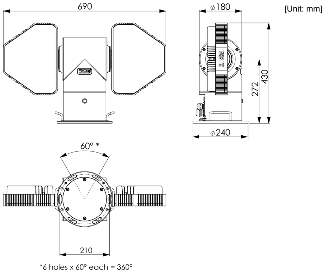
Figure 9 SD-2-135 searchlight
