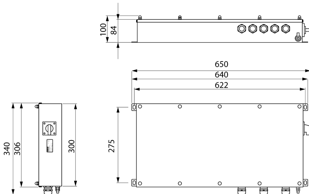
Figure 10 PSUD ballast unit
